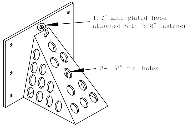
Isometric
